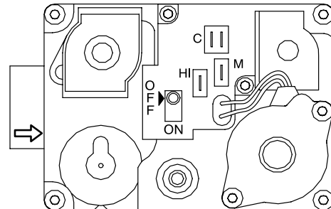
GAS VALVE SHOWN IN OFF POSITION
